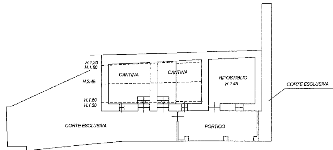
PIANO SEMINTERRATO Hm 2.07
